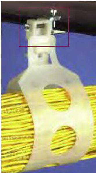
SINGLE LOOP Perpendicular mounting on 1/4" beam clamp
