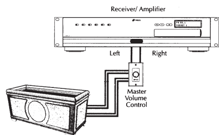
Figure 2. One-speaker stereo, one zone volume control wiring
