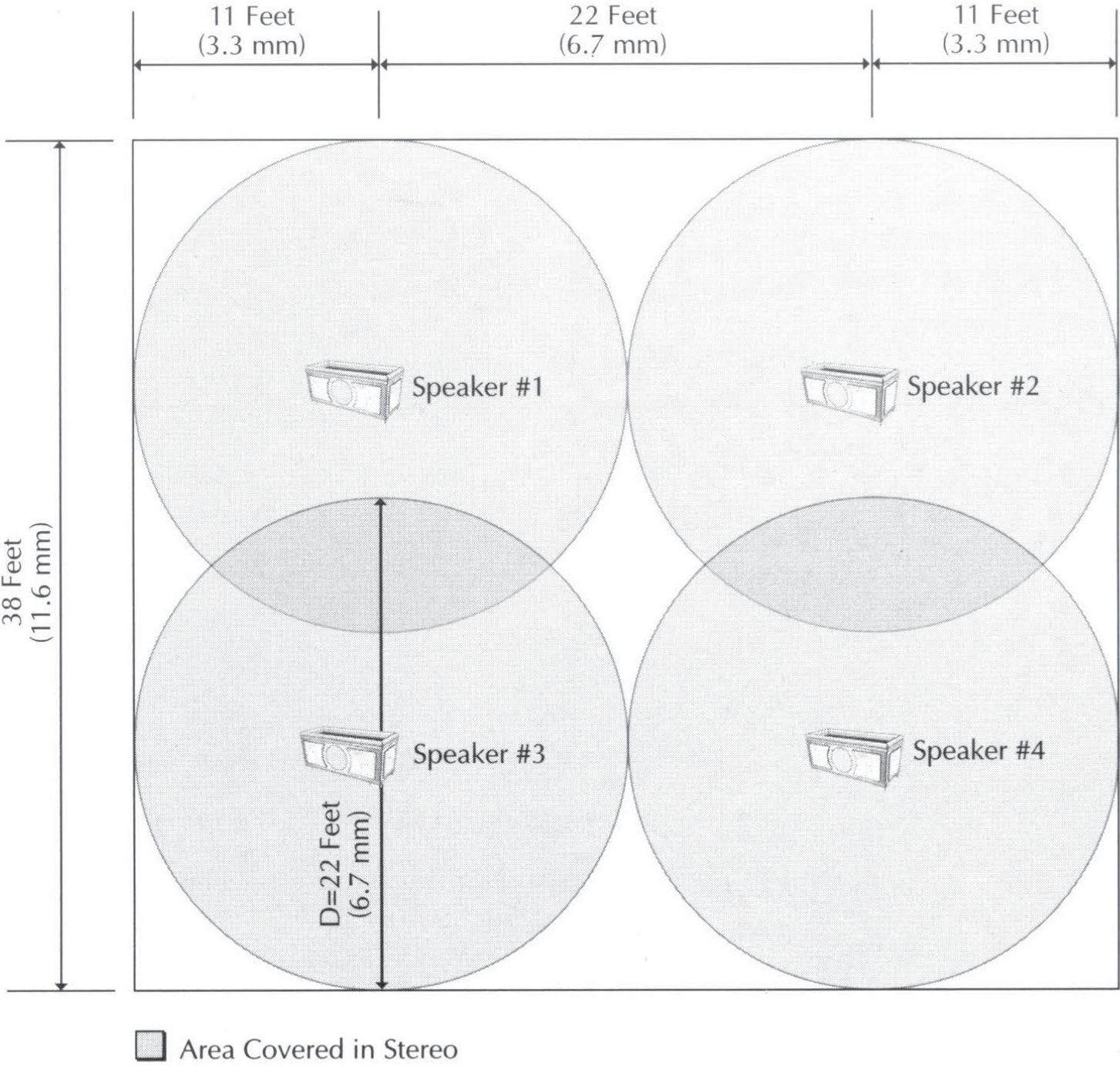
Figure 1. Stereo Coverage – 4 speakers
