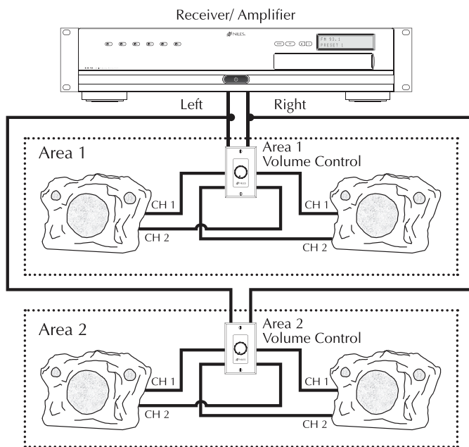
Figure 4b. Two-Speaker Stereo Two Zone VC Wiring
