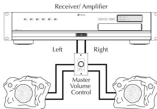
Figure 3b. Two-Speaker Stereo One Zone VC Wiring
