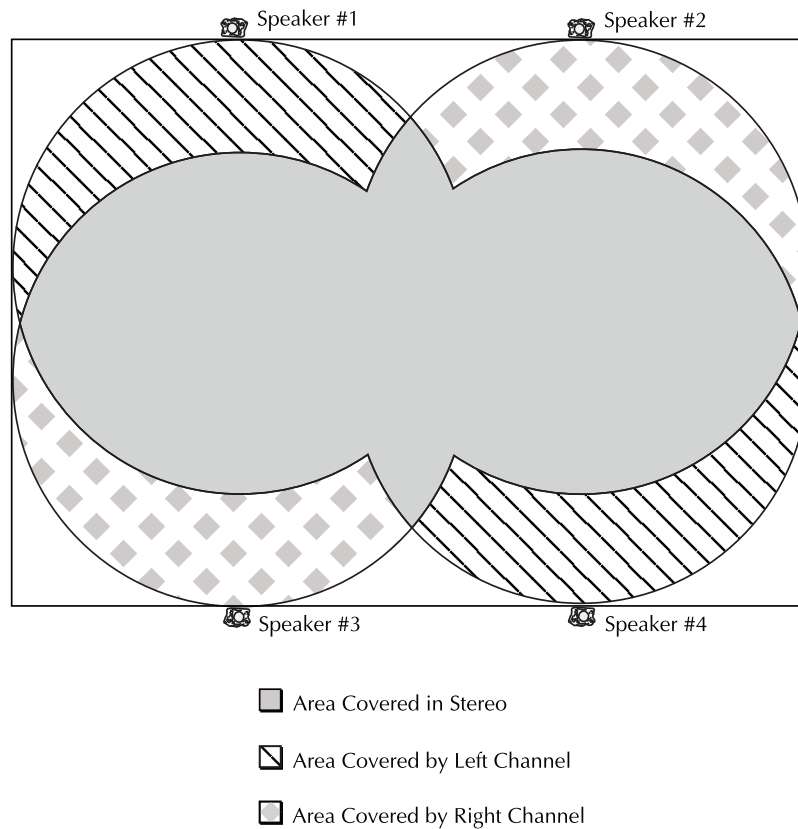
Figure 2. Two-speaker Stereo Coverage – with 4 speakers
