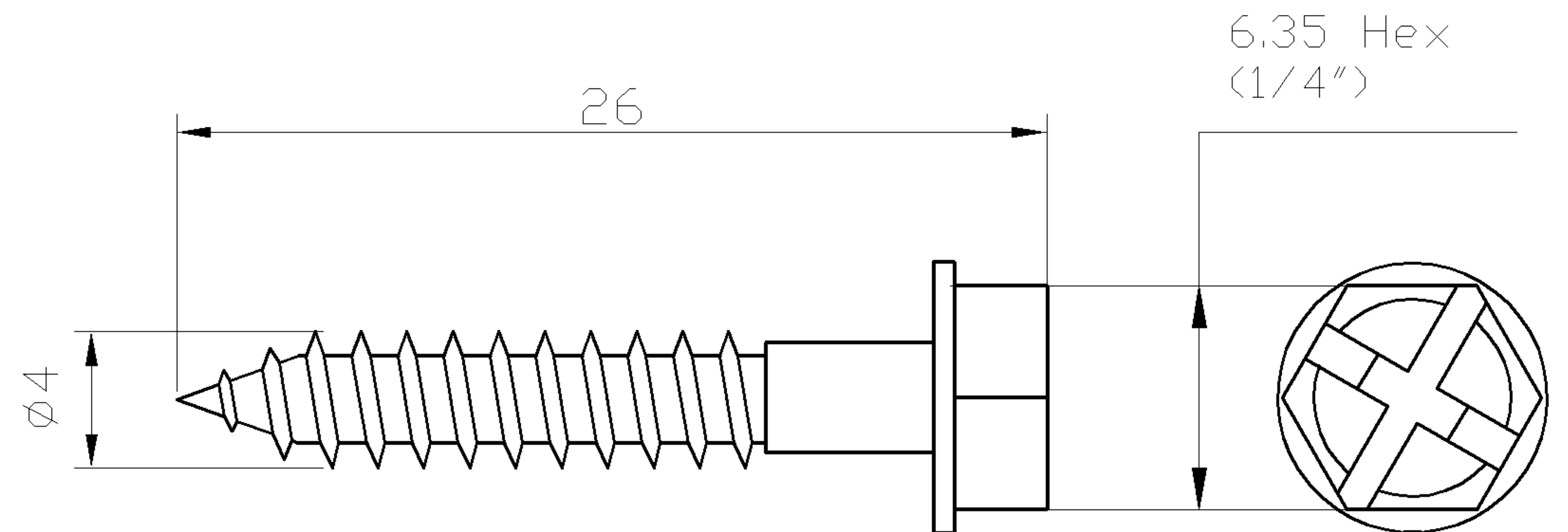
Screw
