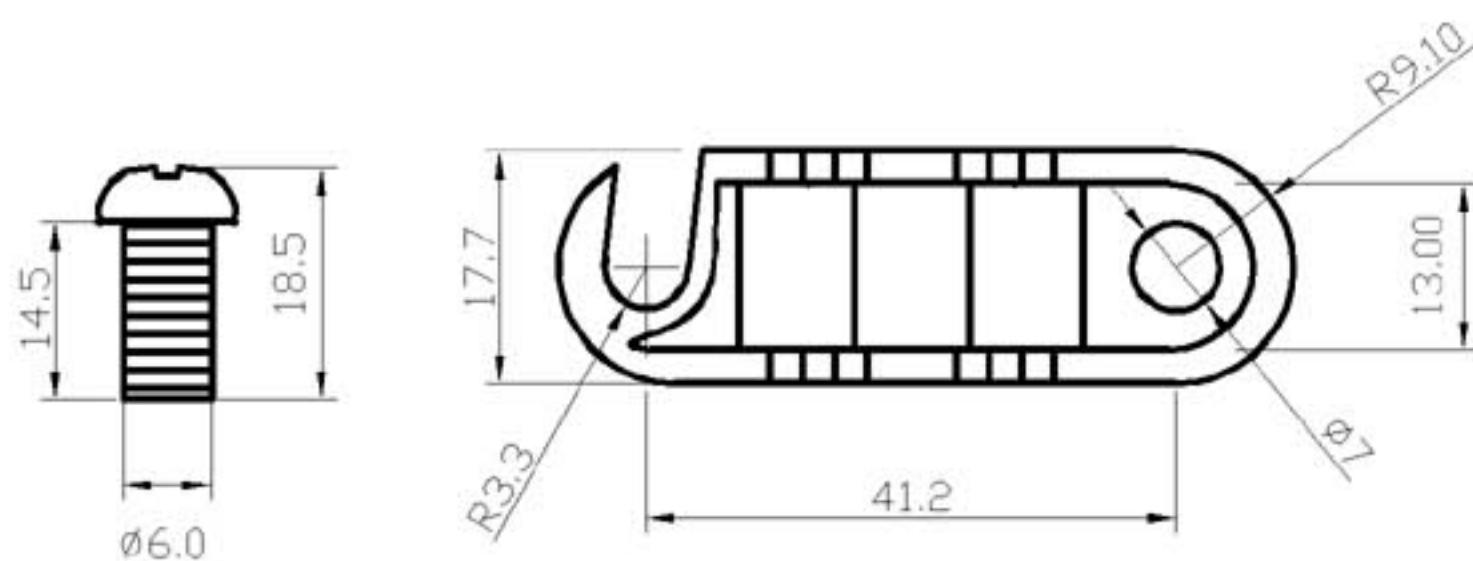
Screw2
