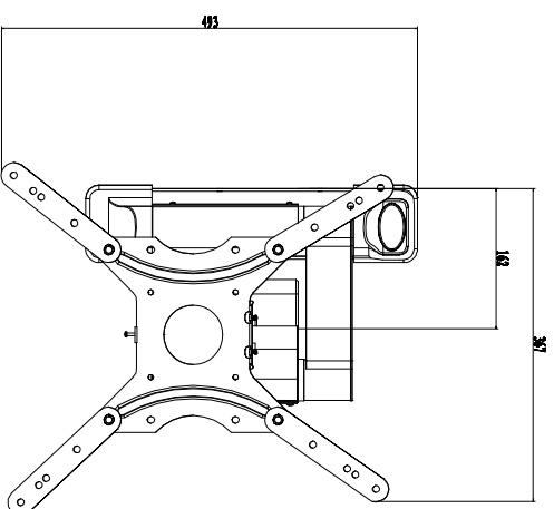
BACK VIEW (Extended with adapter plate and extension bars.)
